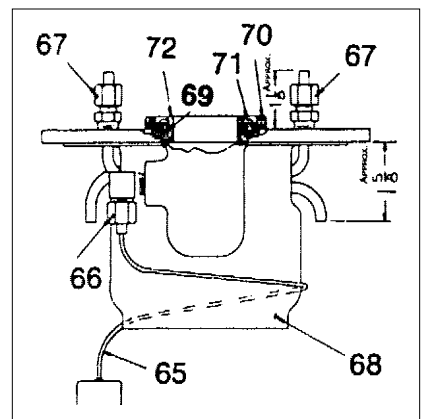
Figure 6 Spider insert.
