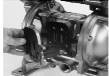
Fig. 3 Pilot valve removal
