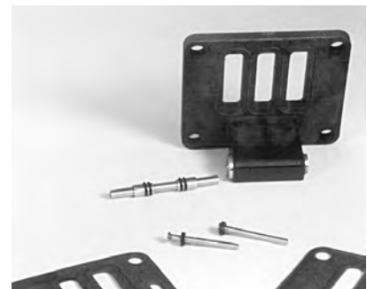
Pilot valve spool and o-rings.
