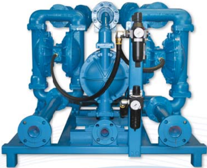
Plate and frame filter press pumping system
