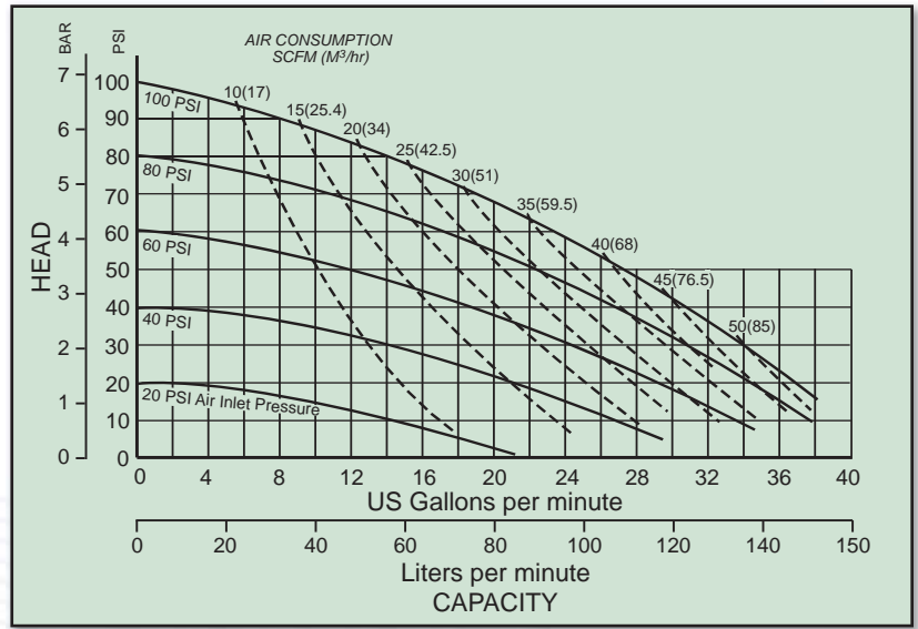
ST1 Metallic Performance Curve
