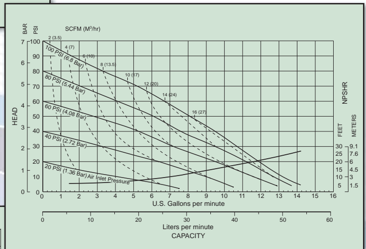
S05 Non-Metallic Performance Curve
