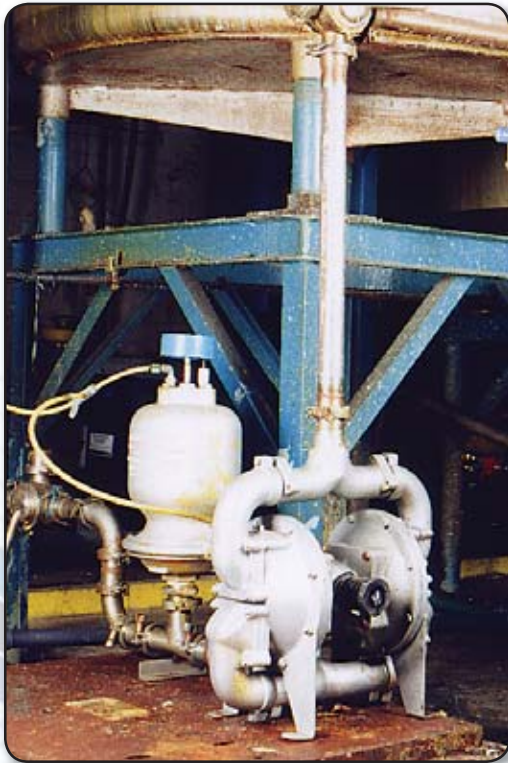
Heavy duty flap valve pump installed on an underflow sludge transfer application.
