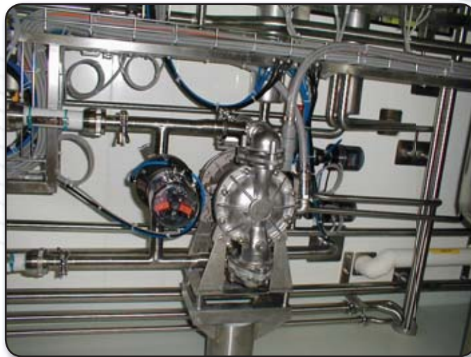
USDA certified ball check valve pump in a clean-in-place, sanitary piping installation.
